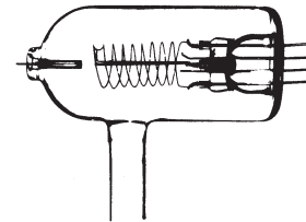
Glass Ion Gauge Tube
