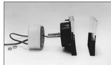
TC Gauge Unassembled
